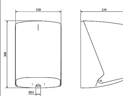
CENTERFEED TOWEL DISPENSER
