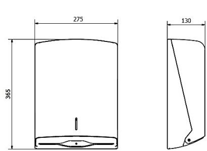
FOLDED TOWEL DISPENSER
