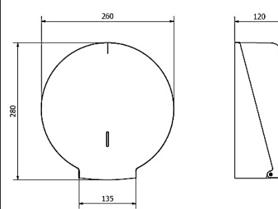
JUMBO TOILET PAPER DISPENSER
