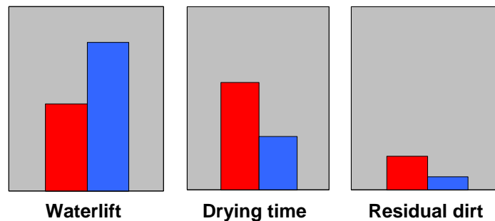
Injection-extraction cleaning with rotating brush
